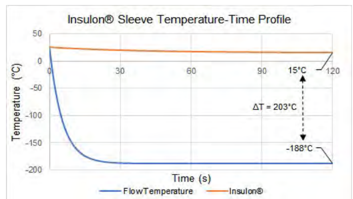
Figure 3: Temperature-time profile of a 6 inch long, 14 gauge Insulon® sleeve carrying liquid nitrogen. Skin temperature reaches steady state at 15°C.
